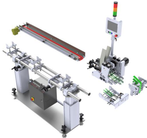
Friction feeder
