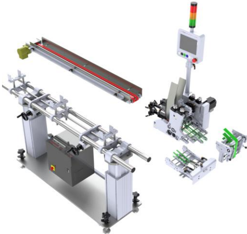
Friction feeder
